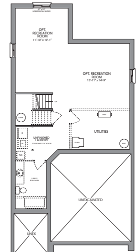
BASEMENT
