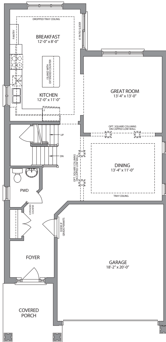
MAIN FLOOR
