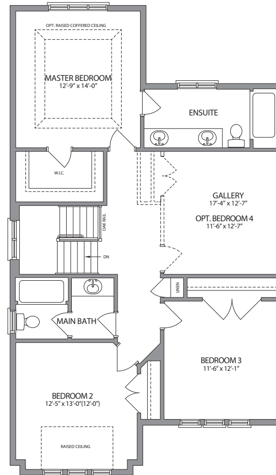
SECOND FLOOR STANDARD
