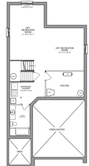
BASEMENT
